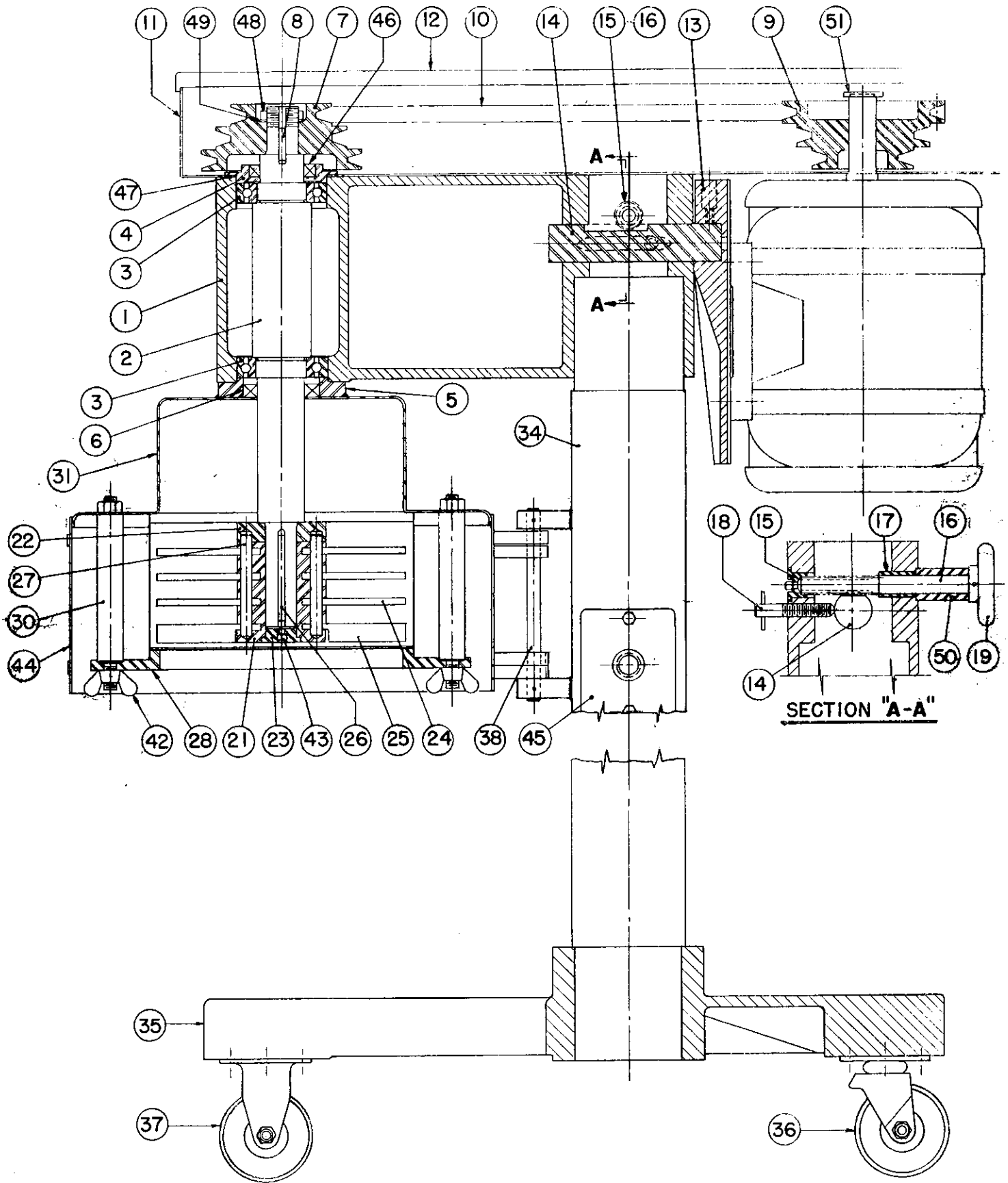
PARTS DRAWING-- 900-44-0 TORNADO MILL (ST-669115 & AFTER)
